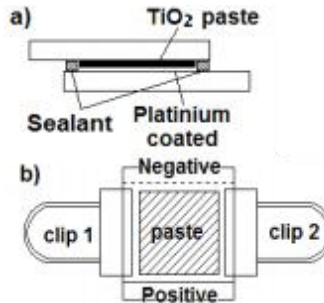
Fig. 5 : The full assemble of DCCS. a) The cross-section view. b) the top view with binder clip on both side.
