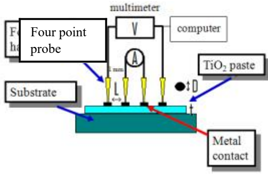
Fig. 4 : Computerized four hand probe diagram to characterize TiO 2 film with metal contact
