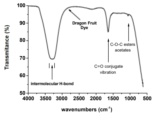
Fig. 7: The FTIR result of dragon fruit dye ranging from 4000 \text{cm}^{-1} to 600 \text{cm}^{-1} .
