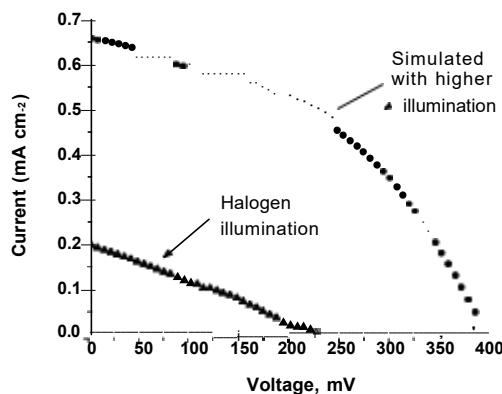
Fig. 9 : The 4th quadrant region result of tested halogen illumination and simulation of higher illumination expected result.
