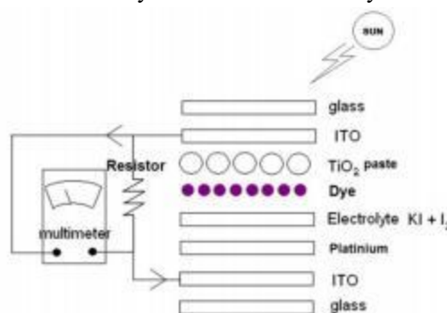
Fig. 1 The cross section assemble consist of ITO glass, \text{TiO}_2 film, dragon fruit dye, electrolyte and platinum layer on ITO glass,
