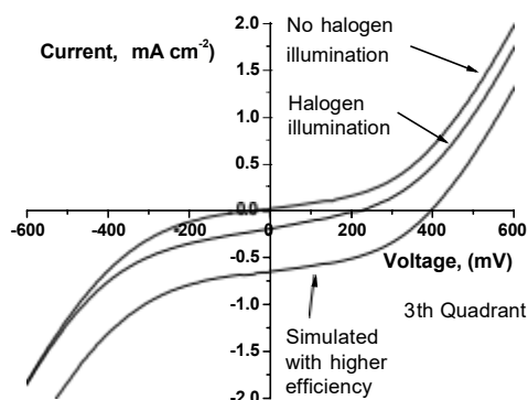
Fig. 8 : The DSSC conversion efficiency test for sample of with and without halogen illumination and simulated reading with higher efficiency.
